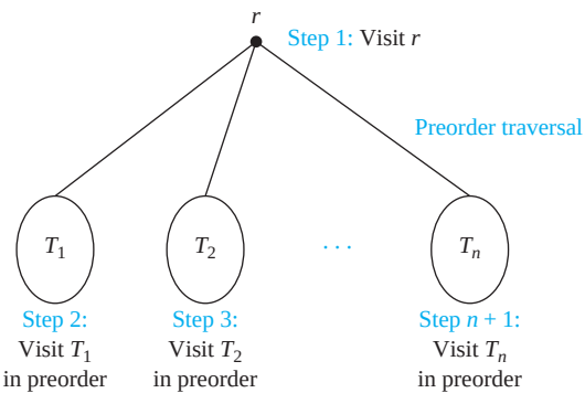
FIGURE 2 Preorder Traversal.
