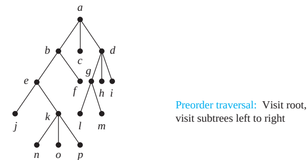
FIGURE 2 Preorder Traversal.
